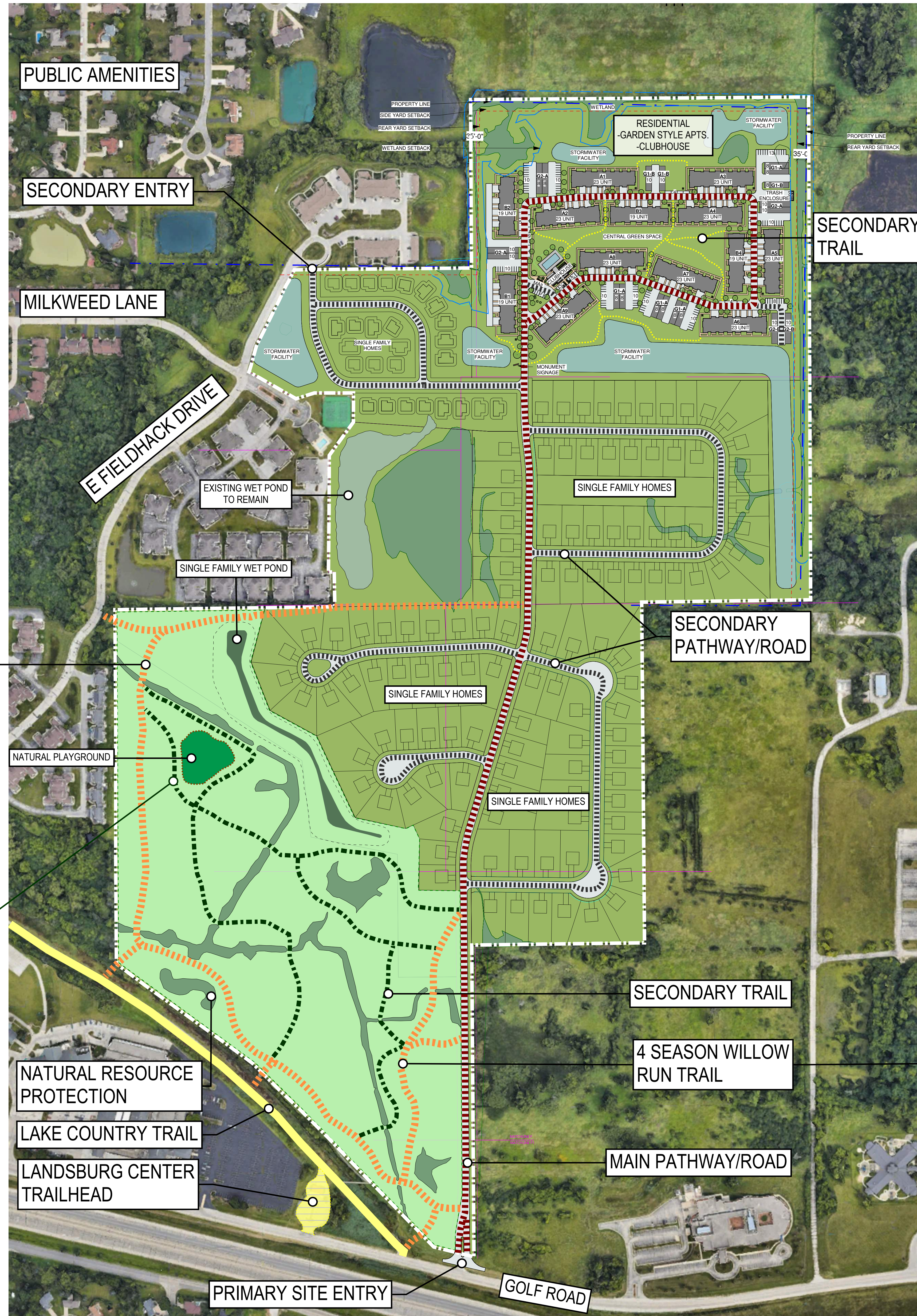
1 OVERALL SITE PLAN - TRAIL EXHIBIT 1" = 200'-0"
